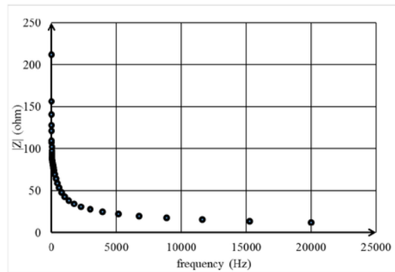
Fig. 2. Bode Plot of Coin Cell
