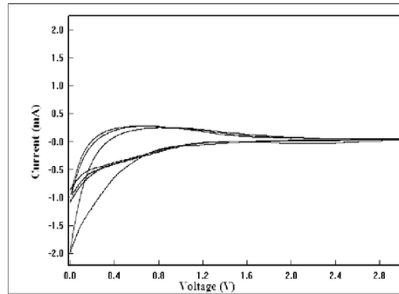
Fig. 3. Voltammogram CV of Coin Cell
