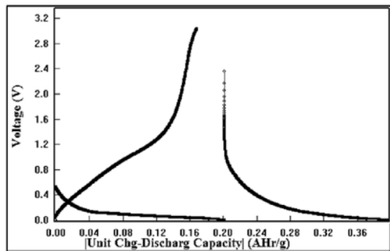
Fig. 4. Charge-Discharge Plot of Coin Cell
