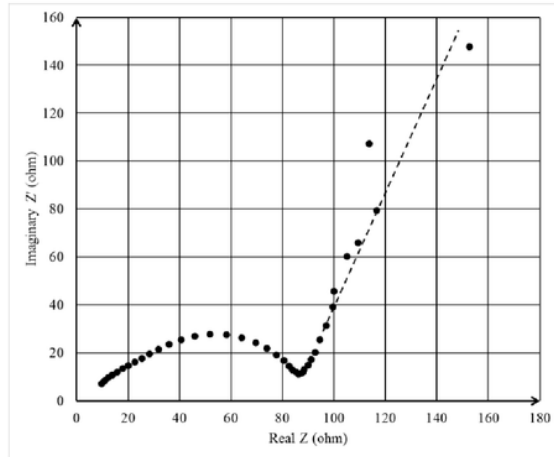
Fig. 1. Nyquist Plot of Coin Cell
